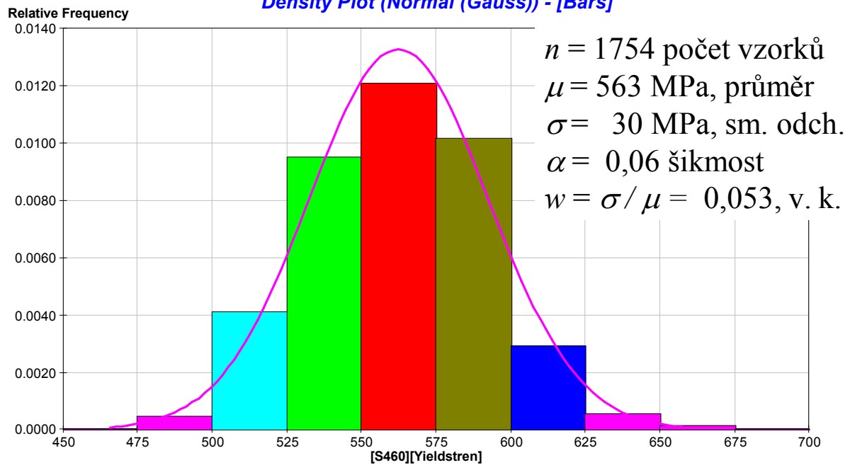
Density Plot (Normal (Gauss)) - [Bars]
