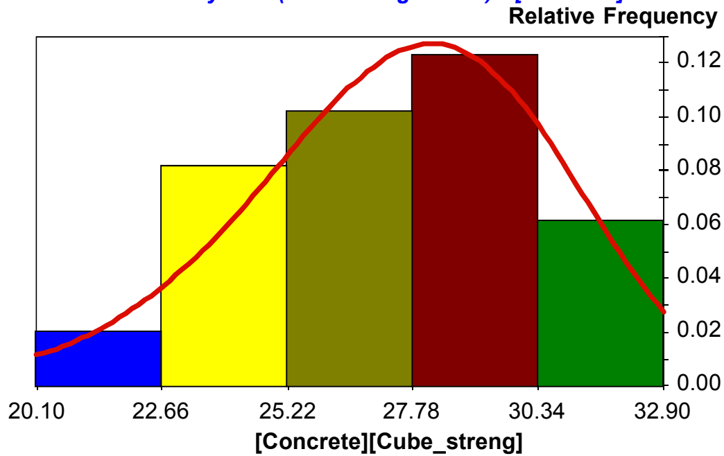
Density Plot (Shifted Lognormal) - [concrete]
